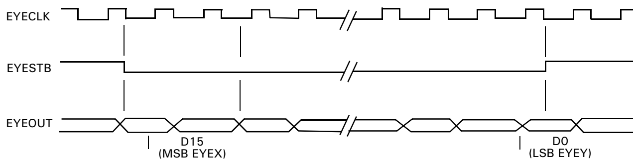
Figure 7. Eye Pattern Port Timing Diagram
