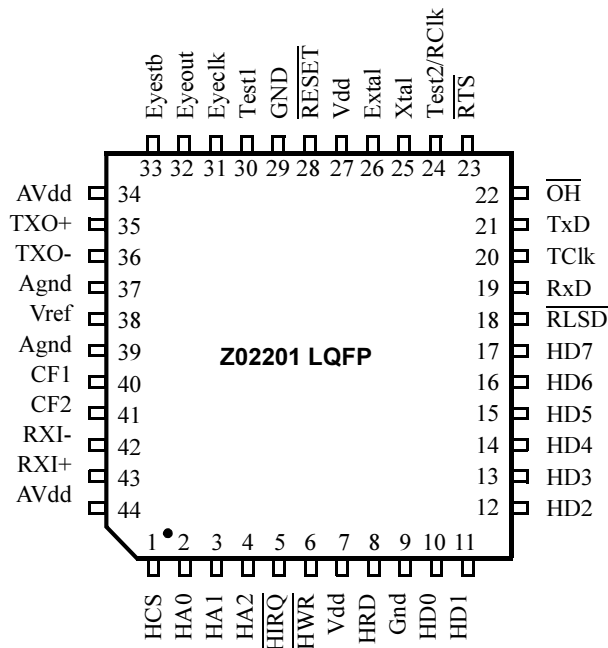
Figure 4. Z02201 44-Lead LQFP Pin Identification
