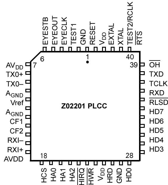
Figure 3. Z02201 44-Lead PLCC Pin Identification
