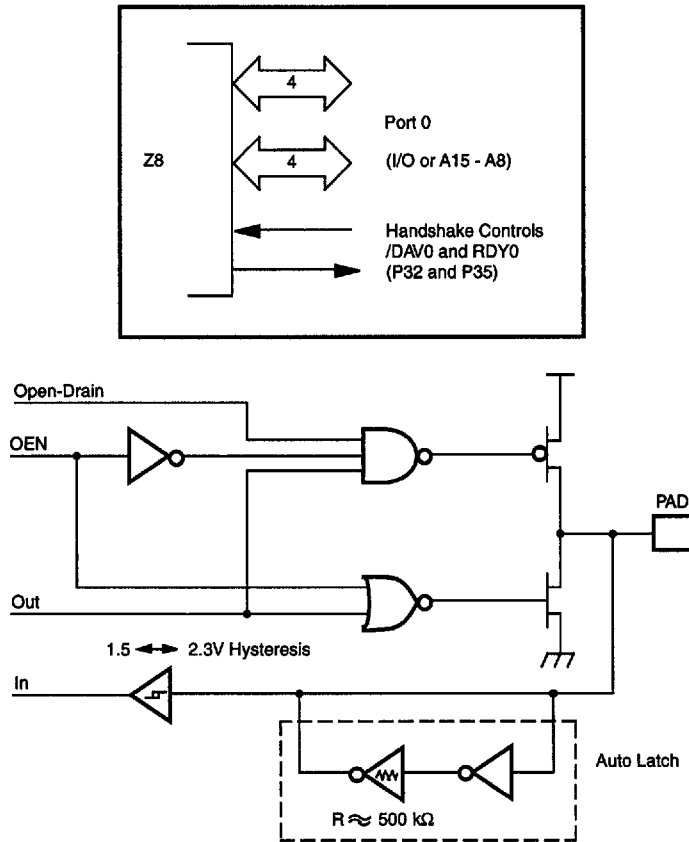
Figure 5-3a. Port 0 Configuration with Open-Drain Capability, Auto Latch, and Schmitt-Trigger
