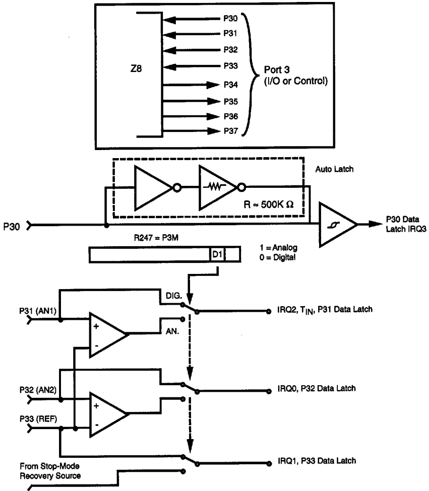
Figure 5-14a. Port 3 Configuration with Comparator, Auto Latch, and Schmitt-Trigger
