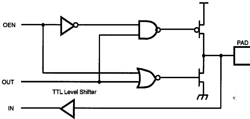
Figure 5-3b. Port 0 Configuration with TTL Level Shifter
