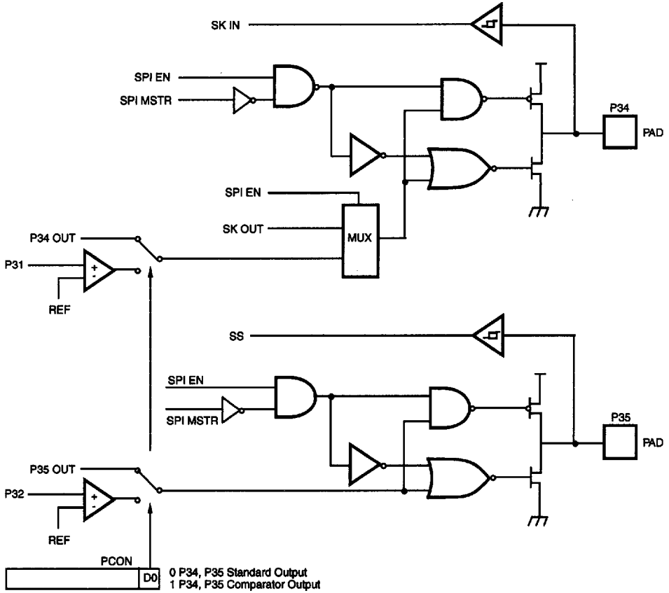
Figure 5-14c. Port 3 Configuration with SPI and Comparator Outputs Using P34 and P35
