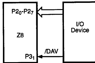
Figure 5-19. Input Strobed Handshake on Port 2
