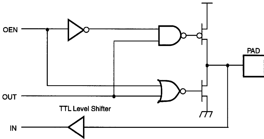
Figure 5-6b. Port 1 Configuration with TTL Level Shifter
