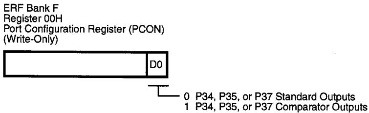
Figure 5-24. Port 3 Comparator Output Selection
