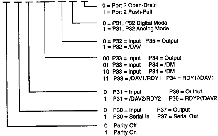
Figure 5-22. Port 3 Mode Reset
