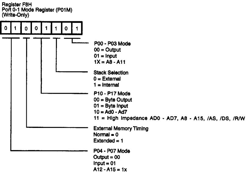
Figure 5-20. Port 0/1 Reset
