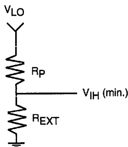
Figure 5-32. Effect of Pulldown Resistors on Auto Latches
