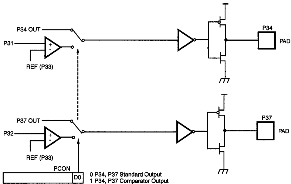
Figure 5-26. Port 3 Configuration
