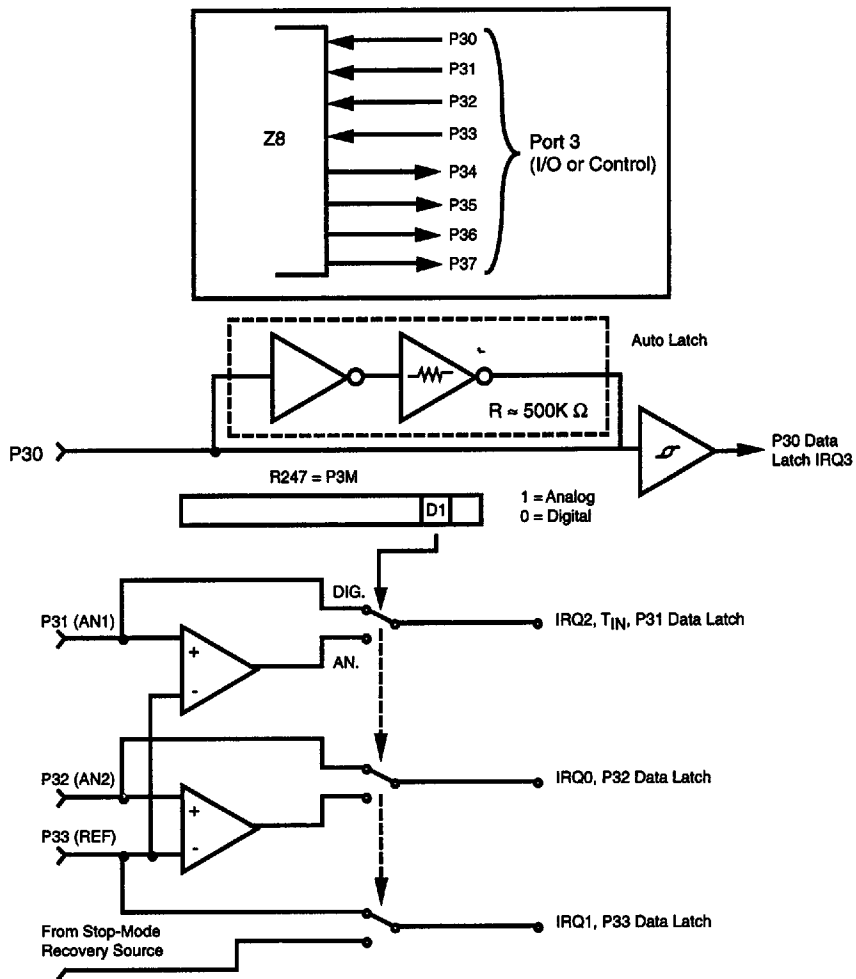
Figure 5-25. Port Configuration of Comparator Inputs on P31, P32, and P33
