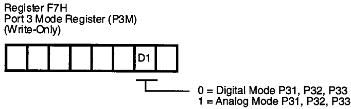
Figure 5-23. Port 3 Input Analog Selection
