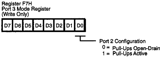
Figure 5-27. Port 2 Configuration
