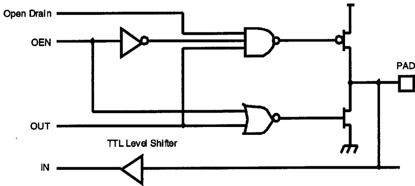
Figure 5-10b. Port 2 Configuration with TTL Level Shifter
