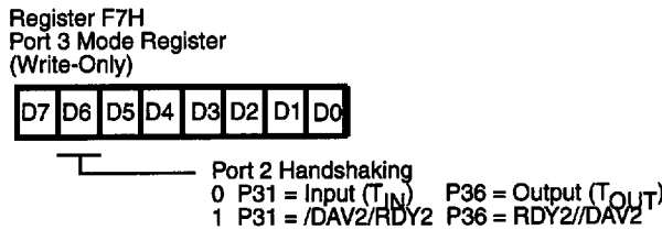
Figure 5-11. Port 2 Handshake Configuration
