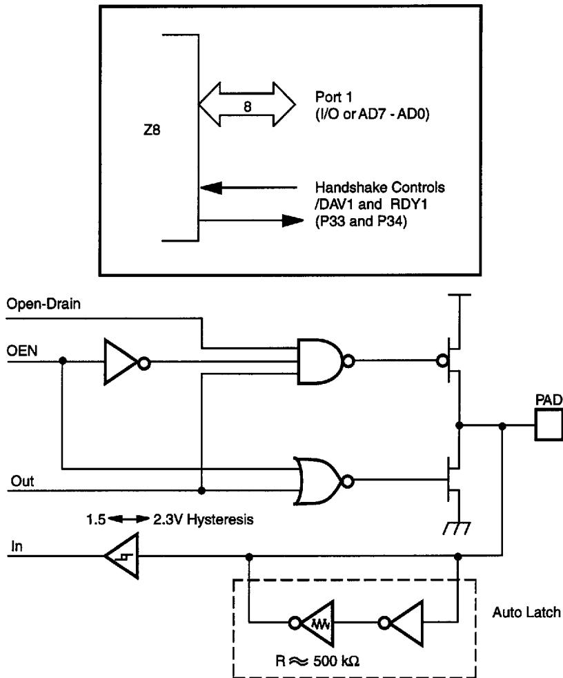
Figure 5-6a. Port 1 Configuration with Open-Drain Capability, Auto Latch, and Schmitt-Trigger
