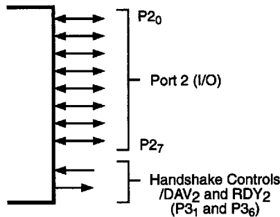
Figure 5-12. Port 2 Handshaking
