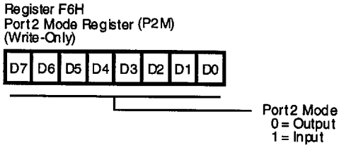
Figure 5-9. Port 2 I/O Mode Configuration
