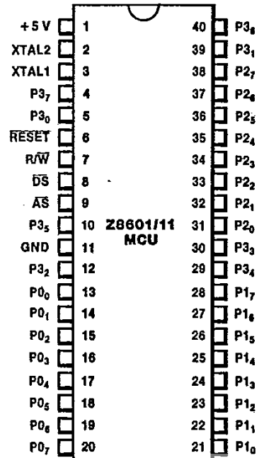
Figure 2a. 40-pin Dual-In-Line Package (DIP), Pin Assignments
