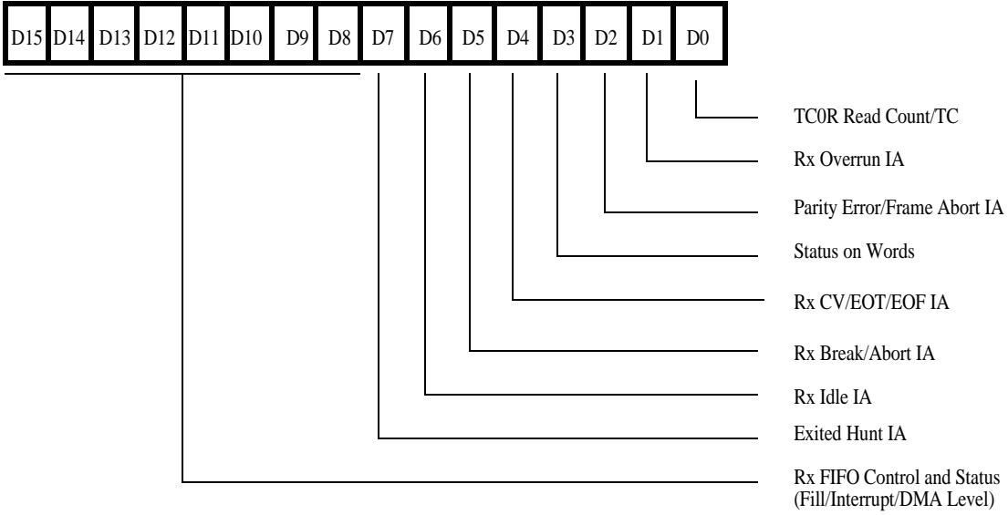
Figure 61. Receive Interrupt Control Register
