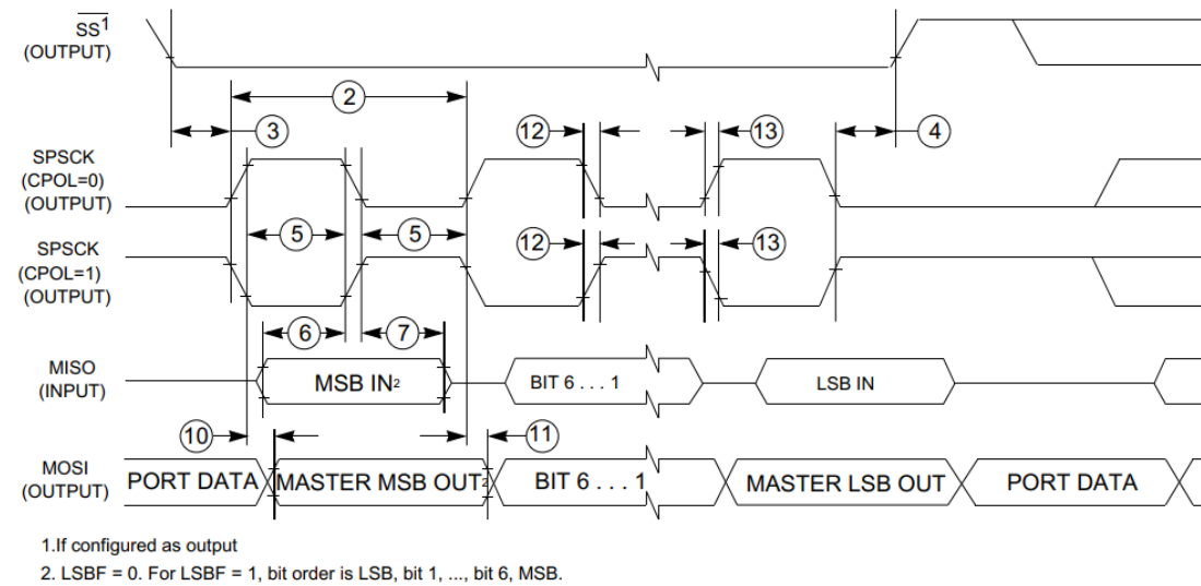
Figure 9. SPI master mode timing (CPHA = 1)
