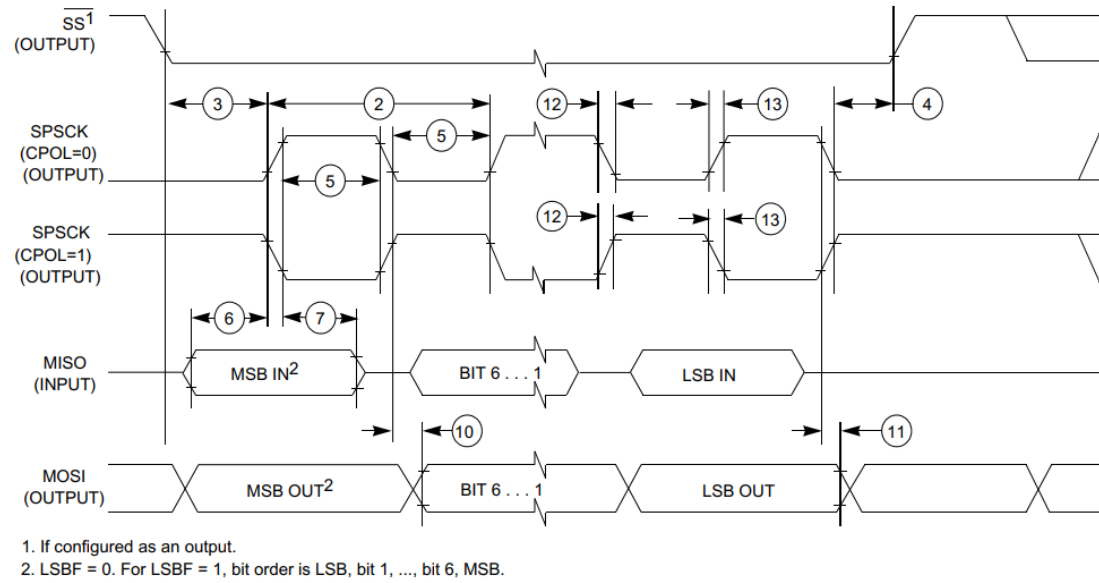
Figure 8. SPI master mode timing (CPHA = 0)
