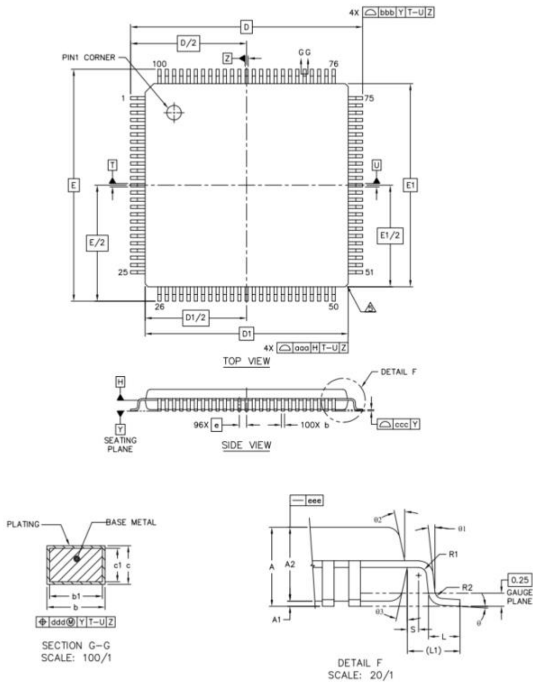
Figure 17. 100-pin products
