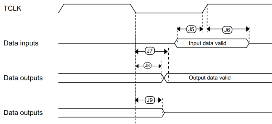
Figure 15. Boundary scan (JTAG) timing
