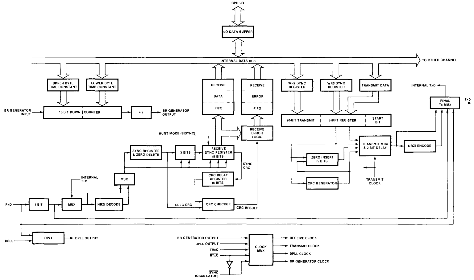
Figure 9. Data Path
