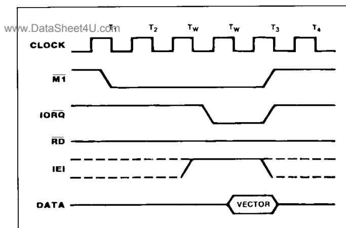
Figure 5c : Interrupt Acknowledge Cycle.
