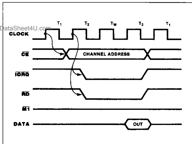
Figure 5a : Read Cycle.
