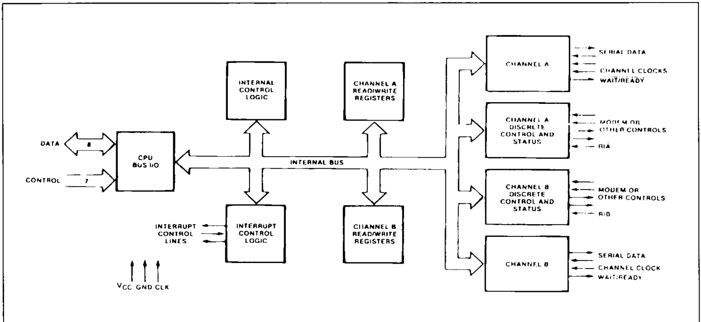
Figure 3 : Block Diagram.
