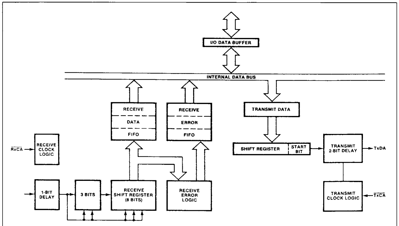
Figure 4 : Data Path.
