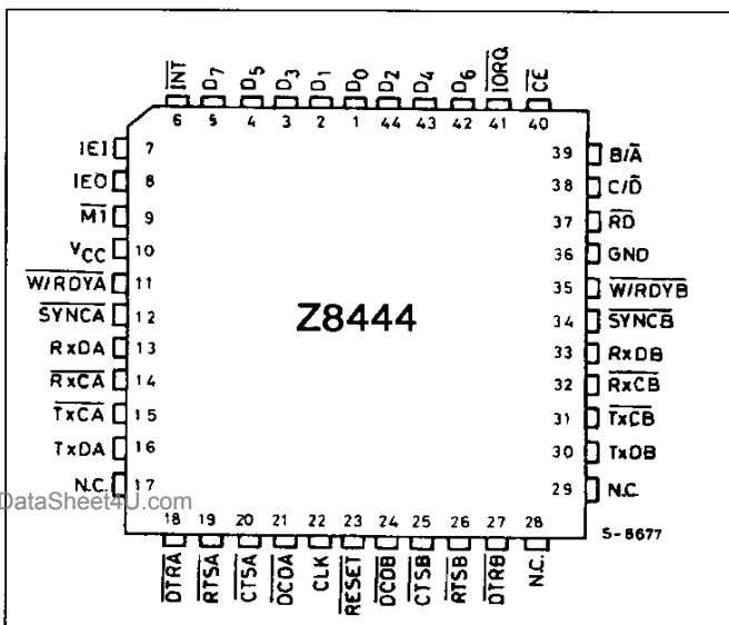
Figure 2 : Chip Carrier Pin Configuration.
