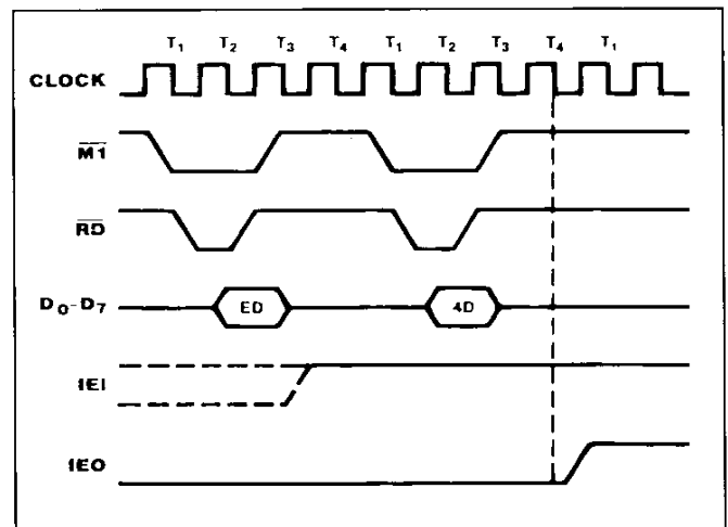
Figure 5d : Return from Interrupt Cycle.
