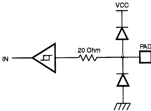
Figure 5. Port 6 Configuration
