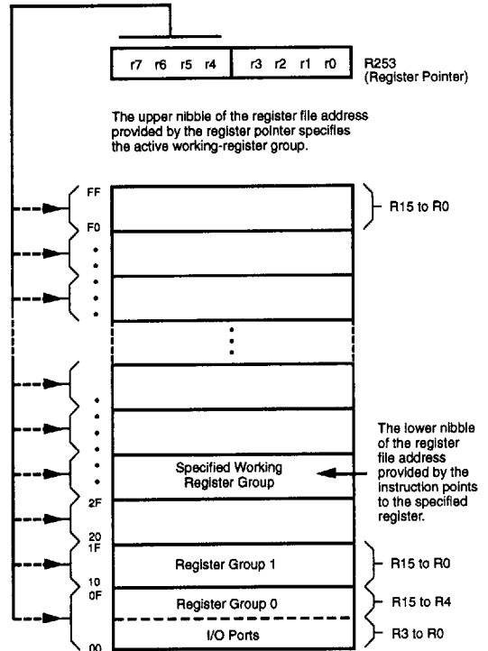
Figure 14. Register Pointer
