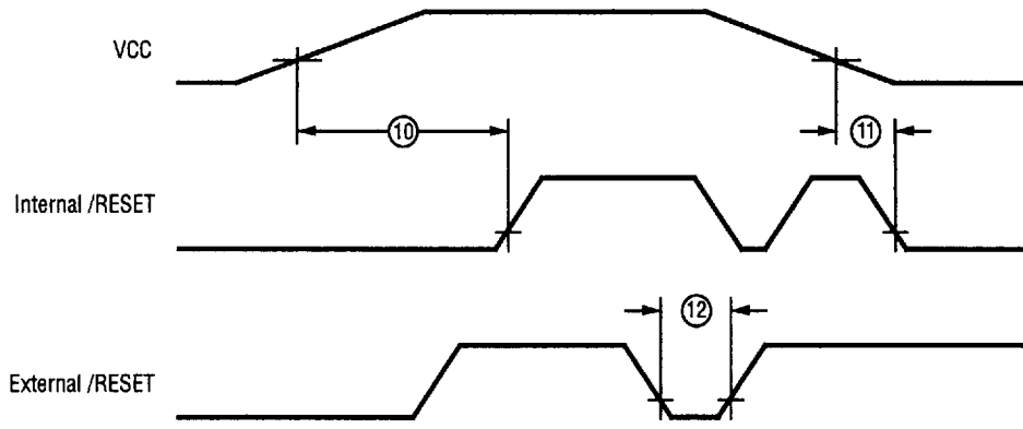
Figure 24. Power-On Reset
