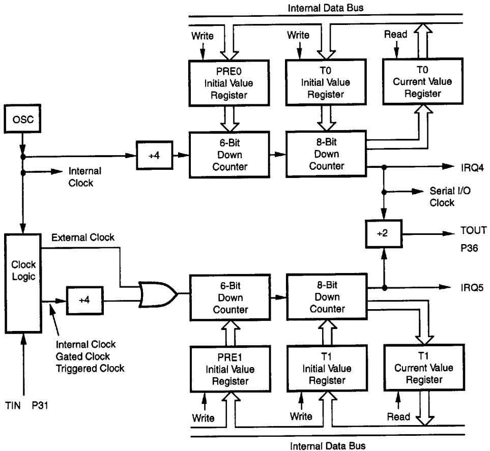
Figure 16. Counter/Timer Block Diagram
