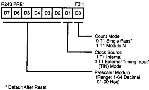
Figure 60. Prescaler 1 Register (F3H; Write Only)
