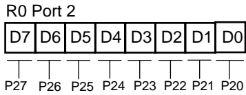
Figure 35. Port 2 Register (Read/Write)
