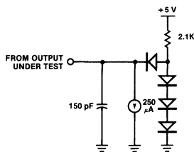
Figure 20. Test Load 1
