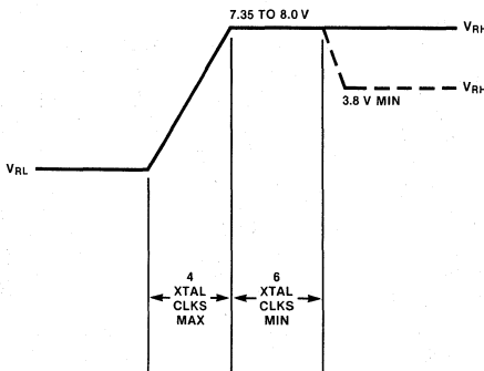
Figure 14. Z8682 \overline{RESET} Pin Input Waveform
