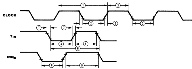
Figure 23. Additional Timing
