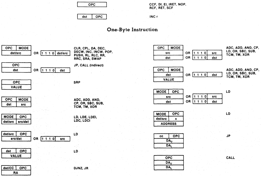
Figure 18. Instruction Formats
