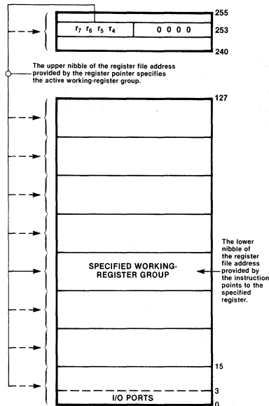
Figure 6. The Register Pointer
