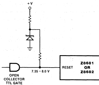
Figure 15. \overline{RESET} Circuit
