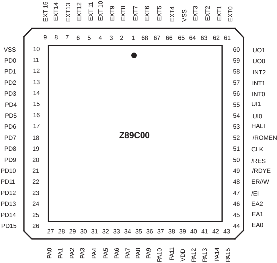
Figure 2. 68-Pin PLCC Pin Assignments
