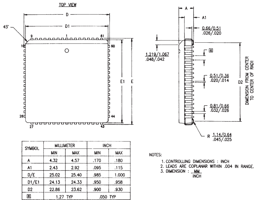
68-Pin PLCC Package Diagram
