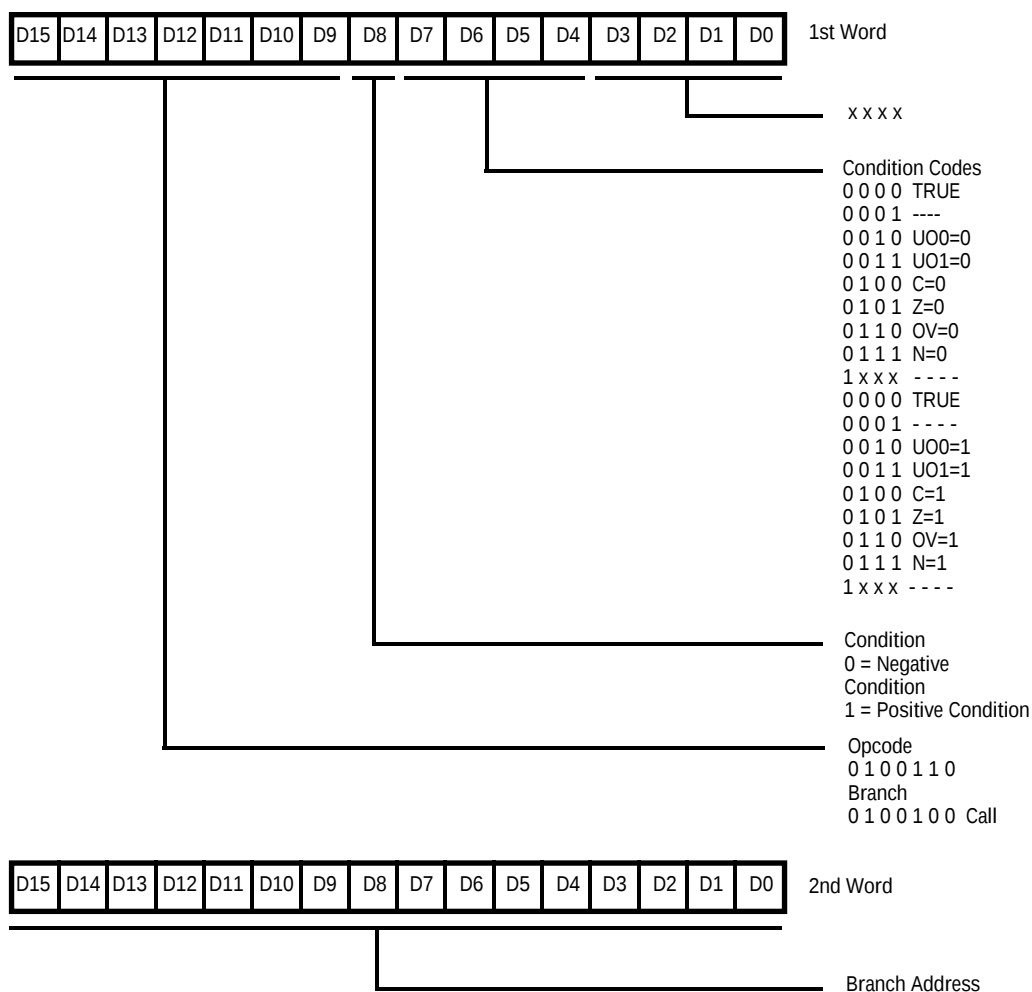
Figure 12. Branching Format
