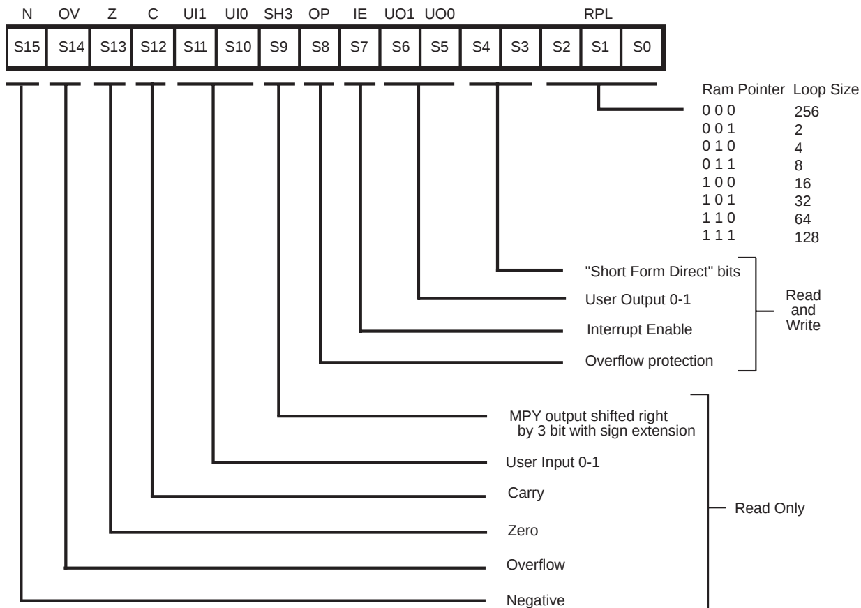
Figure 3. Status Register
