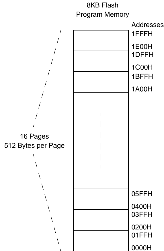
Figure 30. Flash Memory Arrangement
