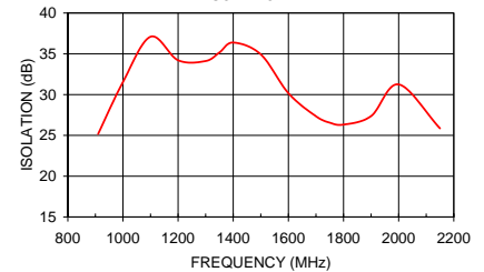
ZAPD-2-22-75+ ISOLATION
