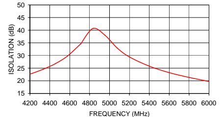
ZAPD-50W ISOLATION
