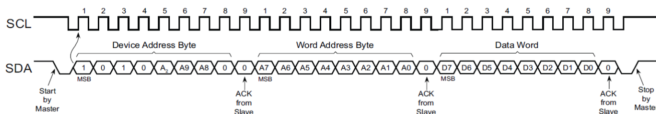
Figure 5-1. Byte Write
