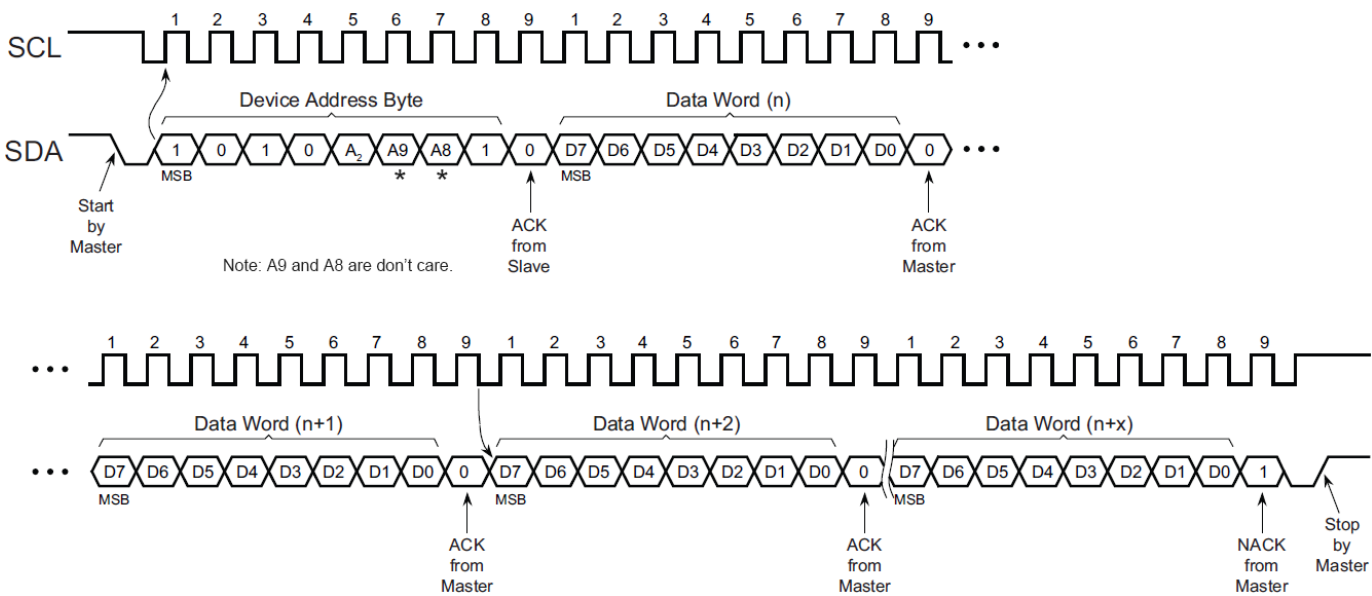
Figure 6-3.Sequential Read
