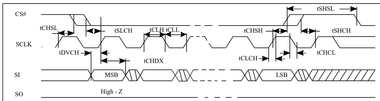
Figure 36. Output Timing
