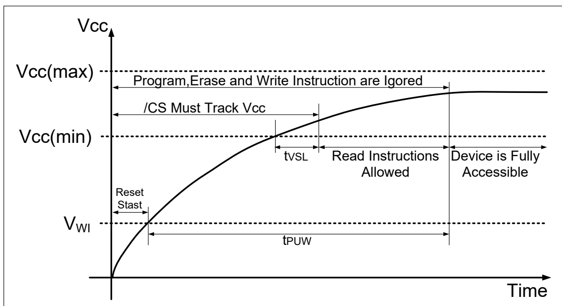
Figure 23, Power-up Timing
