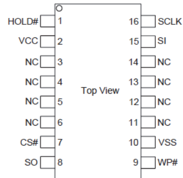
Figure 3.4, 16-LEAD SOP
