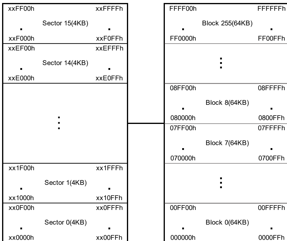
Figure 4, Memory Organization
