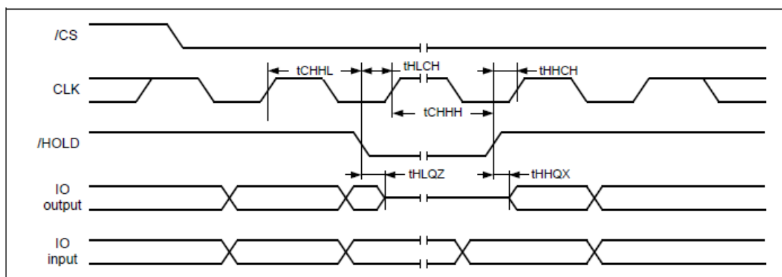
Figure 47, Hold Timing
