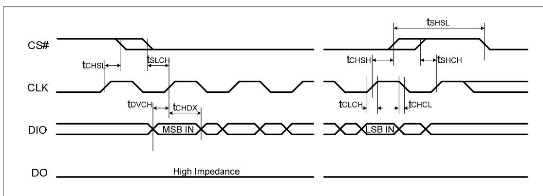
Figure 46, Input Timing
