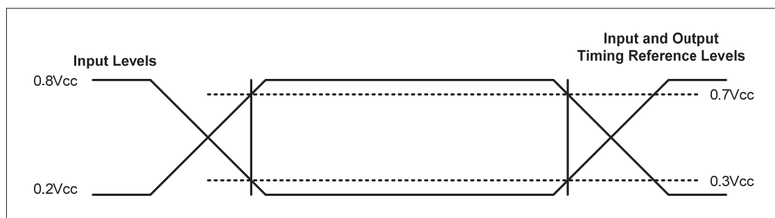
Figure 36, AC Measurement I/O Waveform
