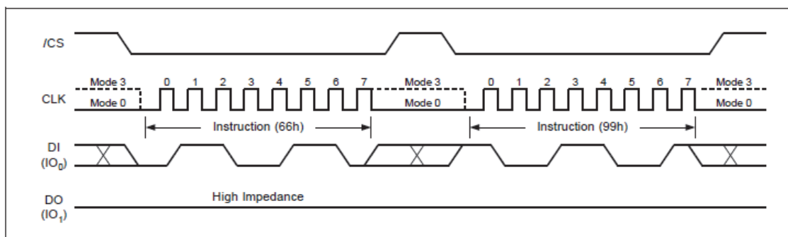
Figure 34. Enable Reset and Reset command Sequence Diagram
