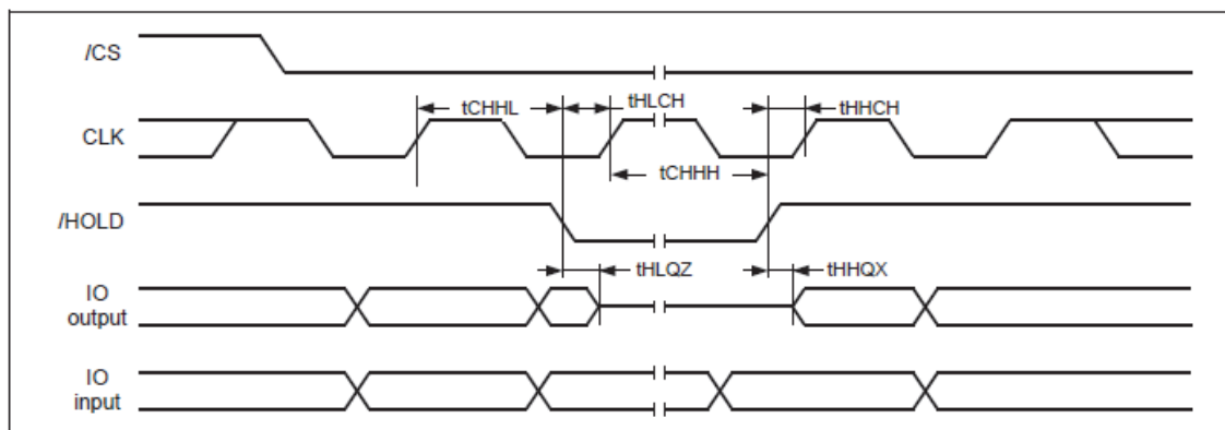
Figure 39, Hold Timing
