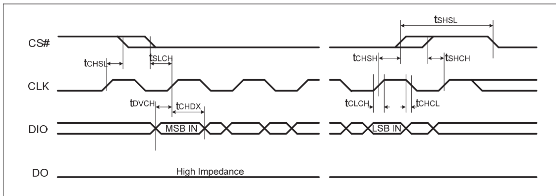
Figure 38, Input Timing
