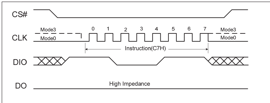
Figure 27, Chip Erase Instruction Sequence Diagram
