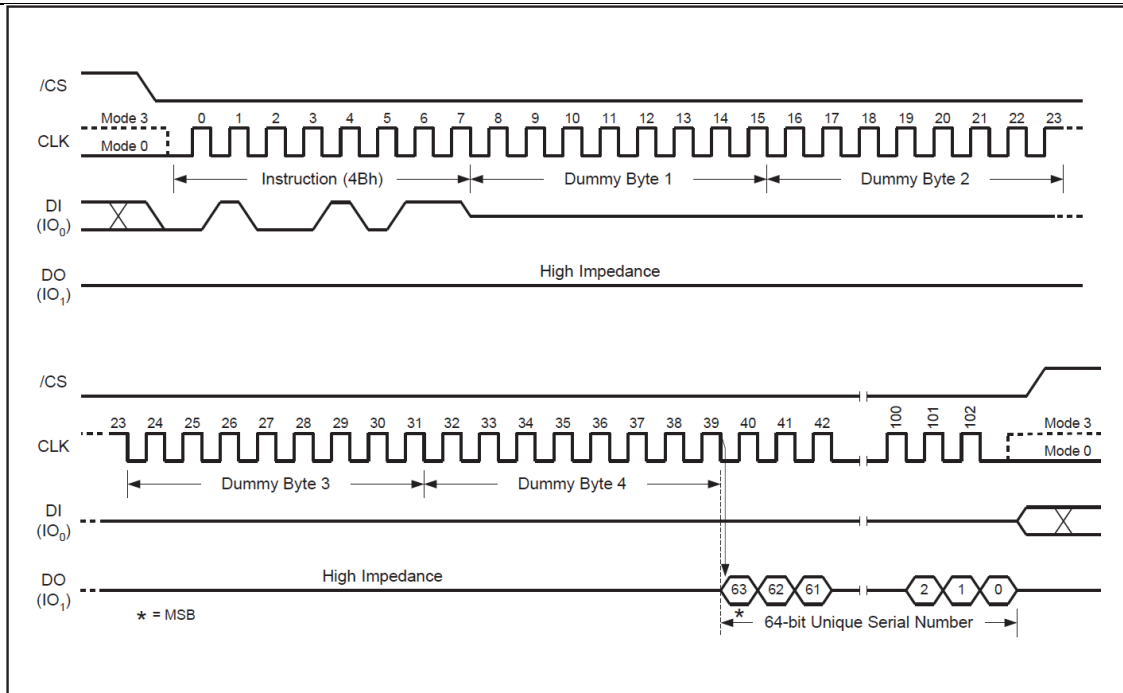
Figure 33, Read Unique ID Number Instruction Sequence Diagram
