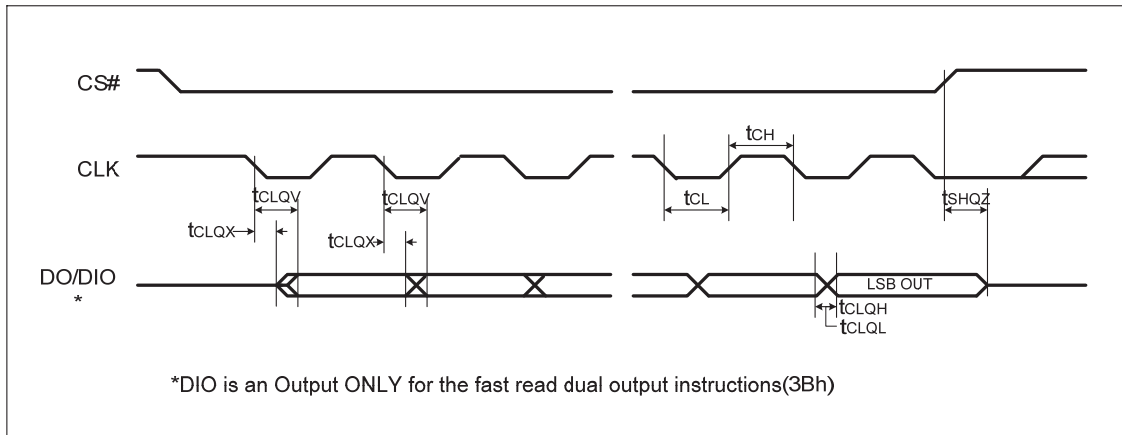
Figure 37, Serial Output Timing
