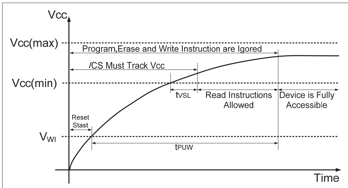
Figure 35, Power-up Timing
