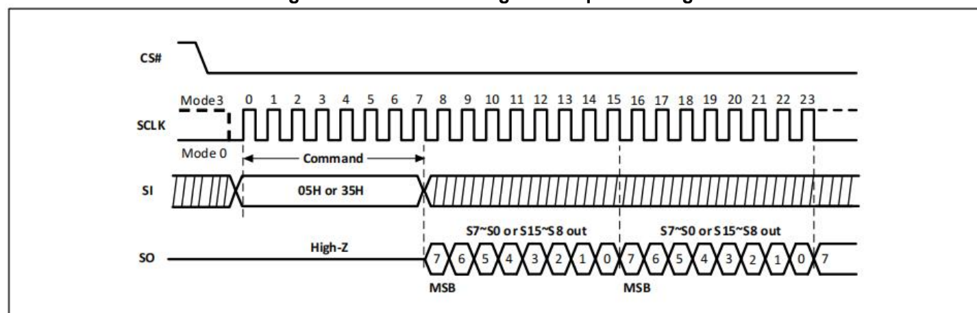
Figure-6. Read Status Register Sequence Diagram
