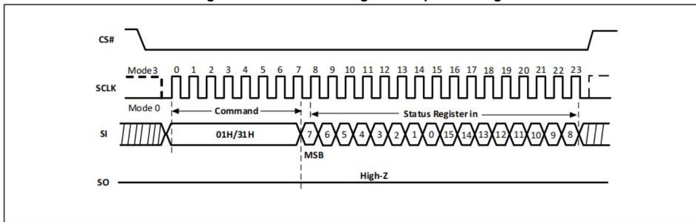
Figure-8. Write Status Register Sequence Diagram
