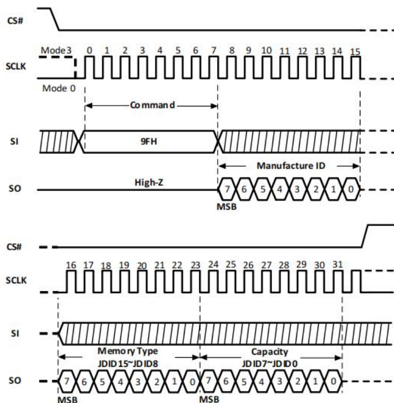
Figure-36. Read Identification Sequence Diagram
