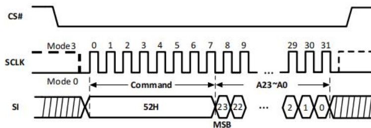
Figure-19. Half Block Erase Sequence Diagram
