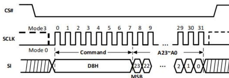
Figure-20. Block Erase Sequence Diagram
