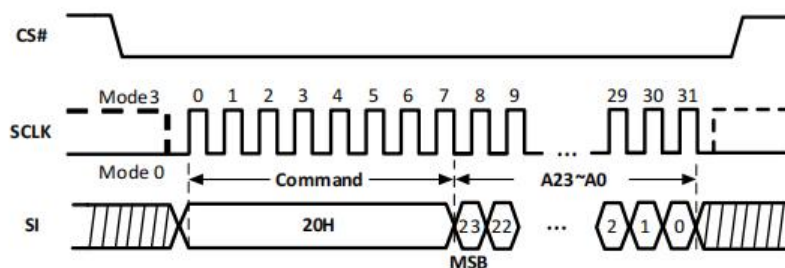
Figure-18. Sector Erase Sequence Diagram
