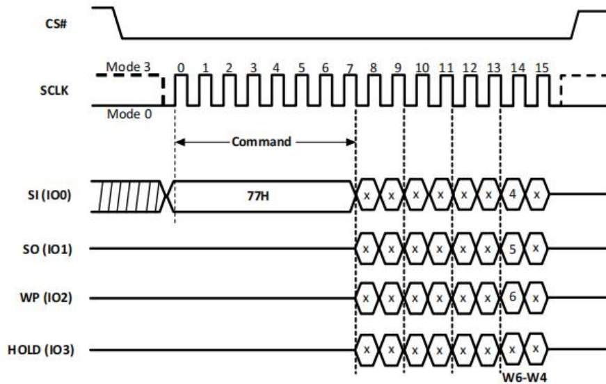
Figure-16. Set Burst with Wrap Sequence Diagram
