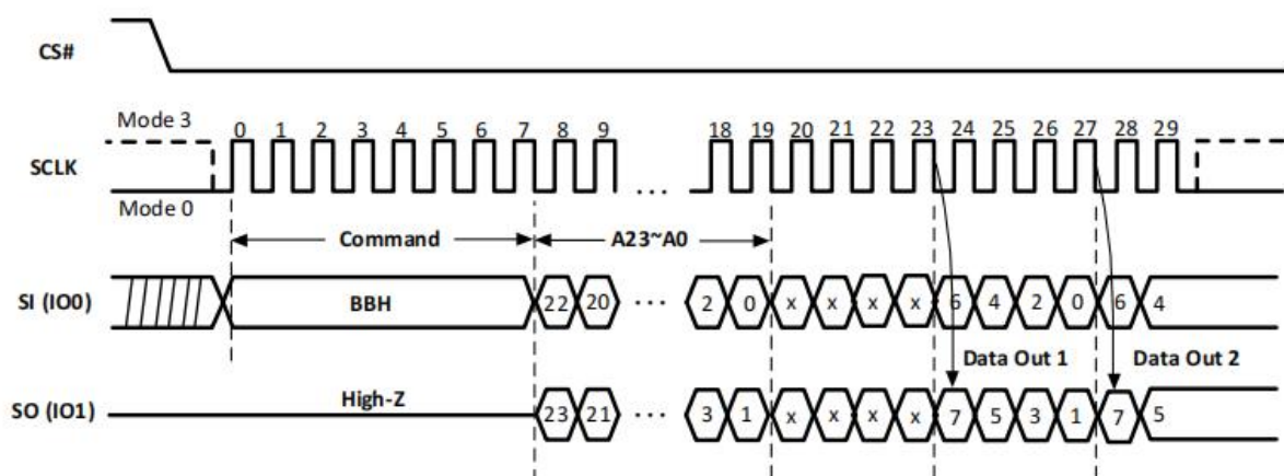
Figure-12. Dual I/O Fast Read Sequence Diagram
