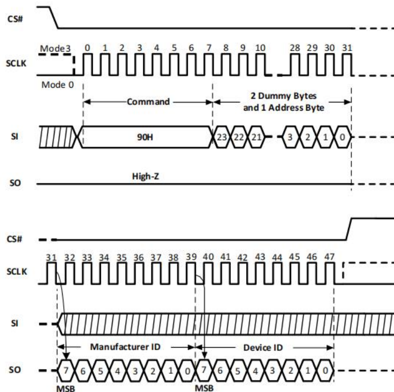
Figure-33. Read Electronic Manufacturer ID & Device ID Sequence Diagram
