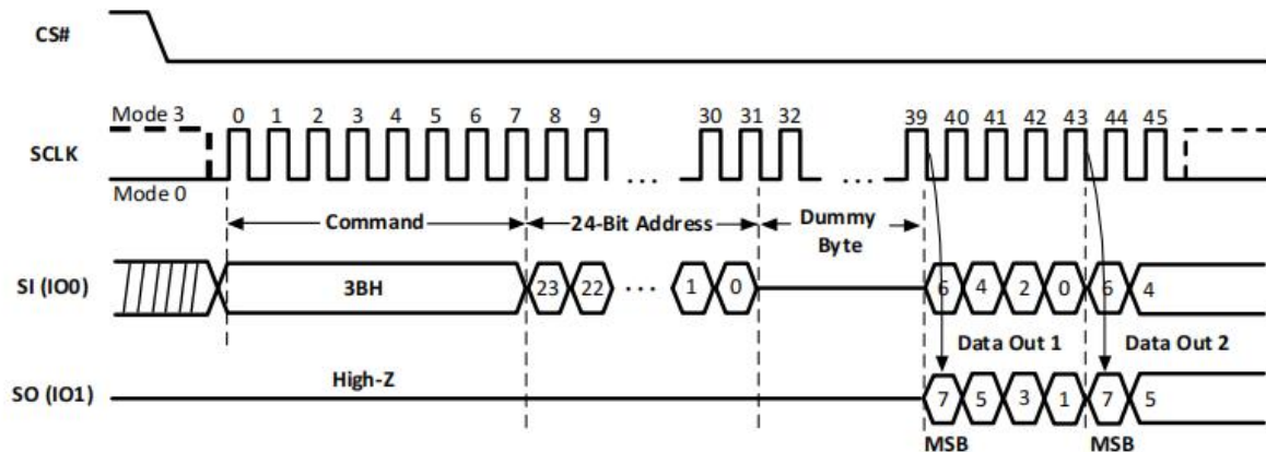
Figure-11. Dual Output Fast Read Sequence Diagram
