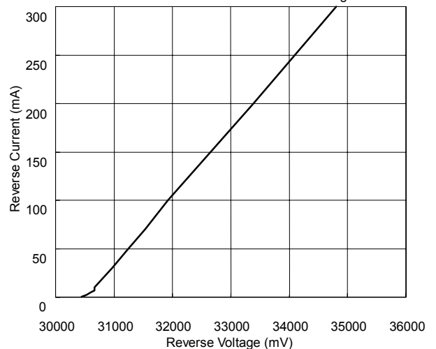
ZD5256B Reverse Current vs Reverse Voltage
