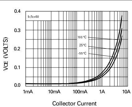
V_{CE(sat)} vs I_C
