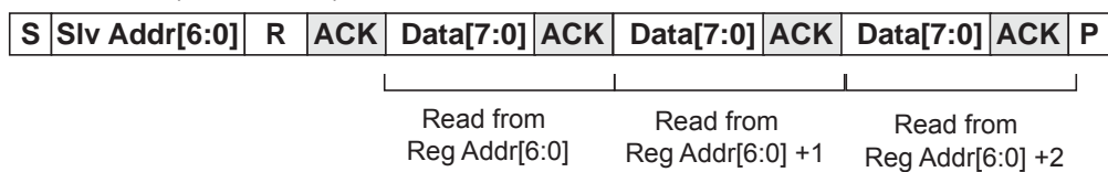
Figure 23 - I 2 C Data Read Burst Mode
