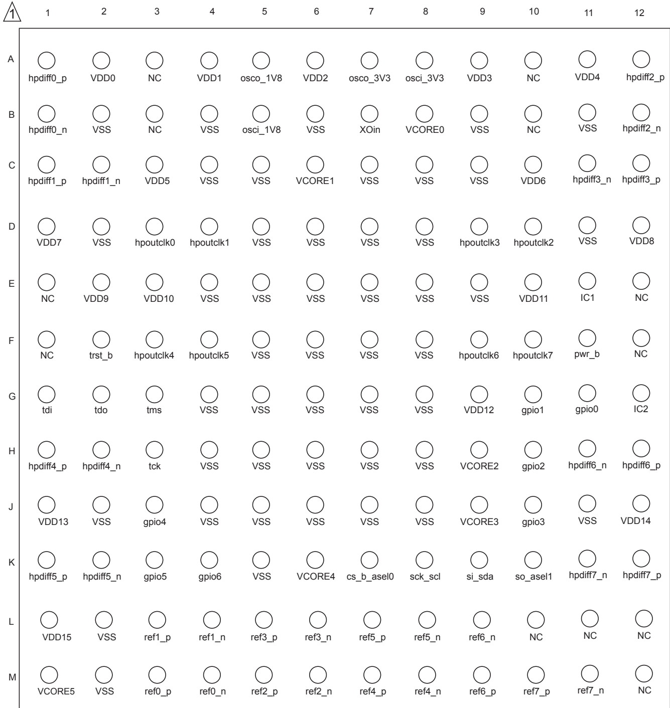
Figure 2 - Package Description
