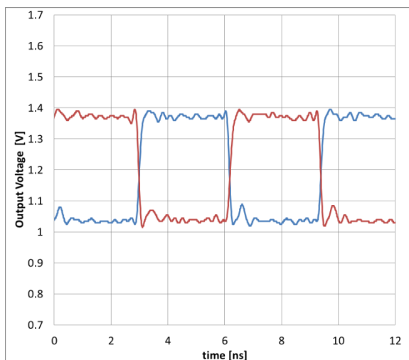
Figure 17. 156.25MHz LVDS
