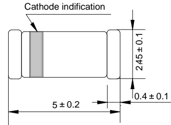
LL- 41 Dimensions in millimeters
