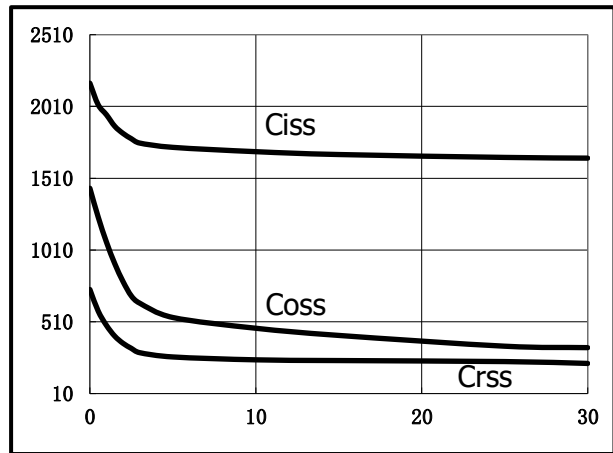
Fig.2 Capacitance Characteristics
