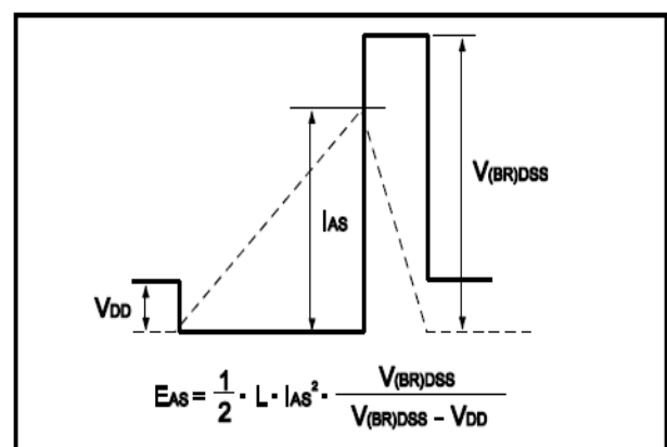
Fig.22 Avalanche Waveform
