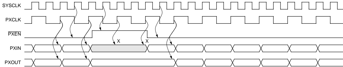
Figure 6. \text{PXCLK} = \text{SYSCLK}/2
