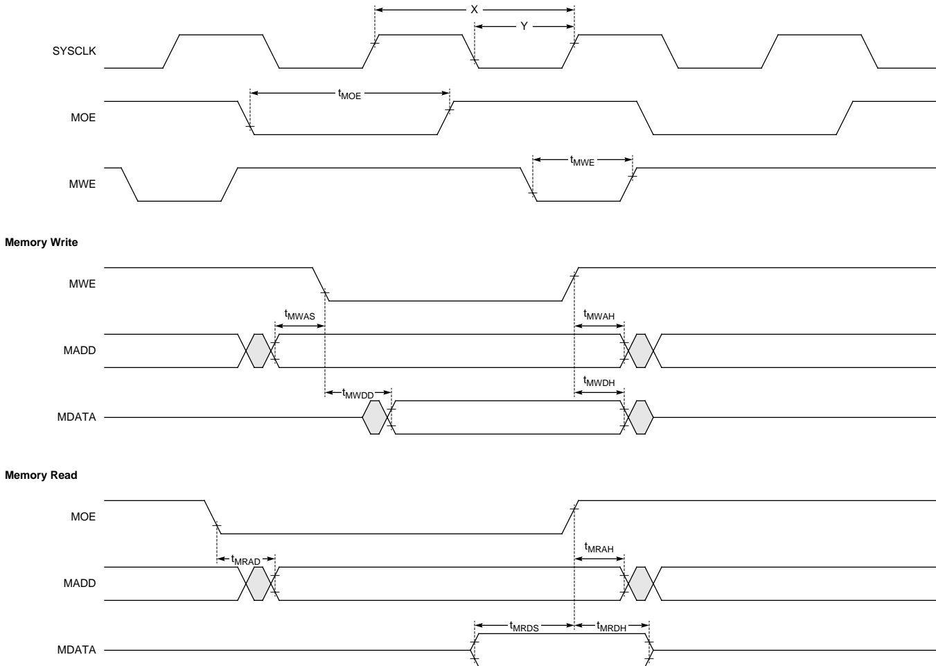
Figure 40. Memory Interface Timing
