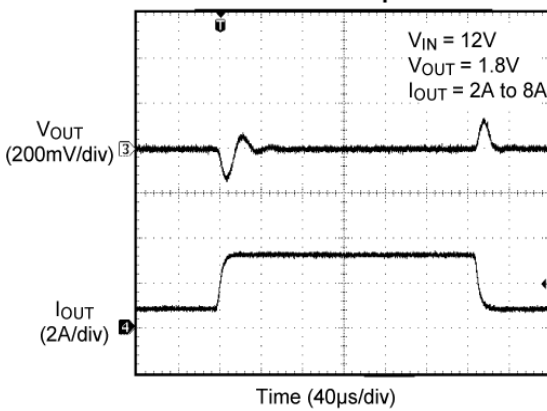
Transient Response
