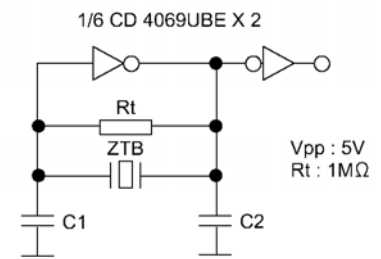
Figure 3) Test Circuit
