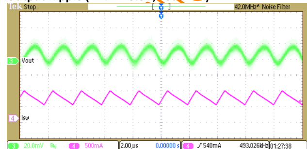
Output Ripple (12V => 3.3V, Load=0A)
