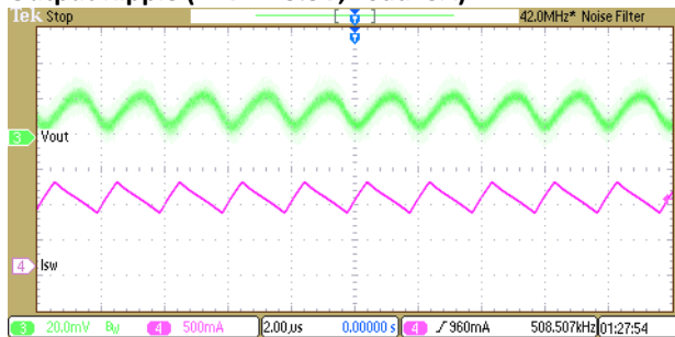
Output Ripple (12V => 3.3V, Load=1A)
