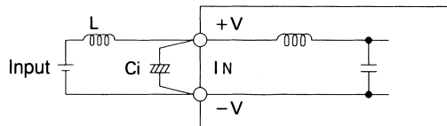
Fig. 3.1 Connection method of capacitor at input terminal
