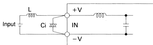
Fig. 3.1 Connecting method of capacitor at input terminal
