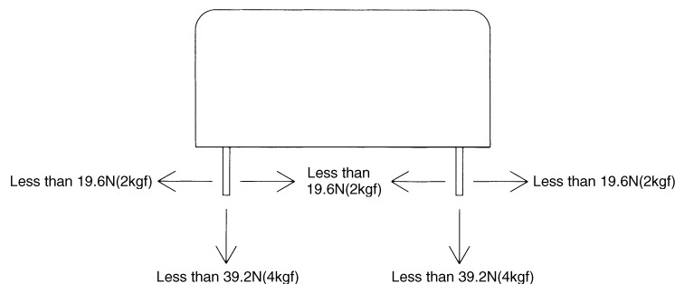
Fig. 9.1 Stress onto the pins
