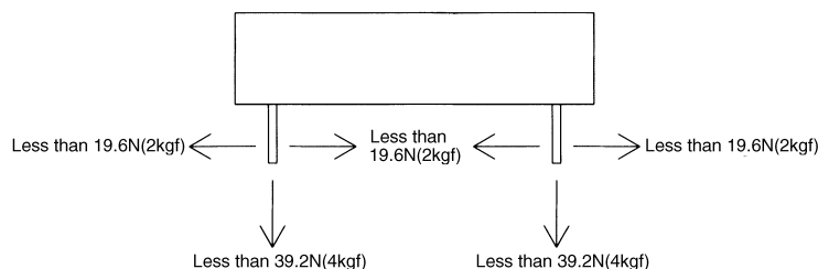
Fig. 9.1 Stress onto the pins
