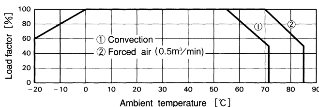
Fig. 5.2 Derating curve
