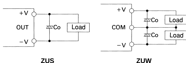
Fig. 3.2 Connecting method of external capacitor at output terminal
