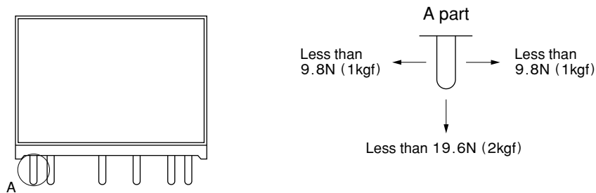
Fig. 9.1 Stress onto the pins
