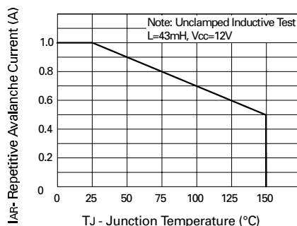
Maximum Repetitive Avalanche Current v Junction Temperature
