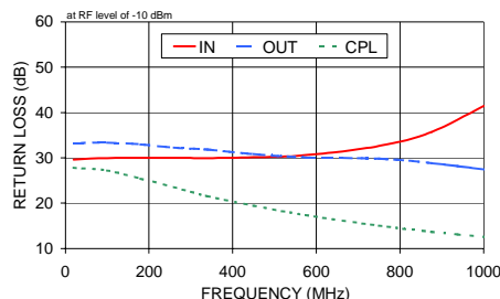
ZX30-20-4 RETURN LOSS
