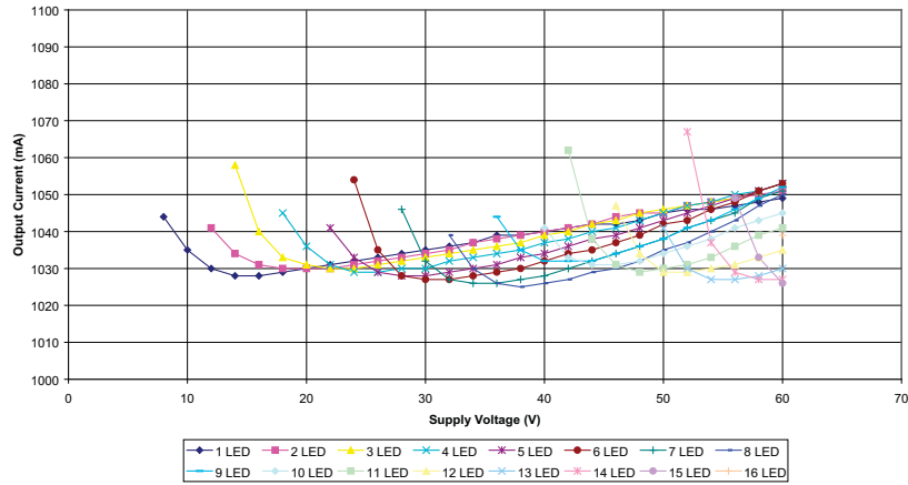
ZXLD1362 Output Current L=150μH
