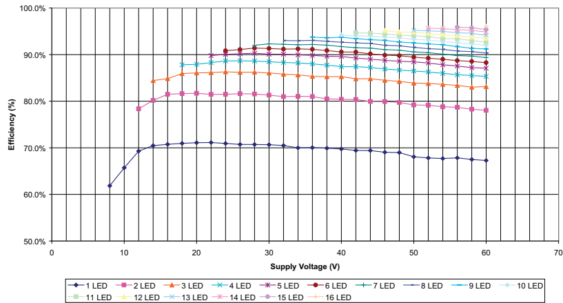
ZXLD1362 Efficiency L=150μH
