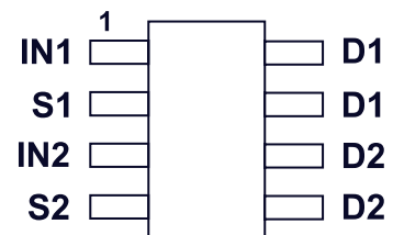
SM8 Package
