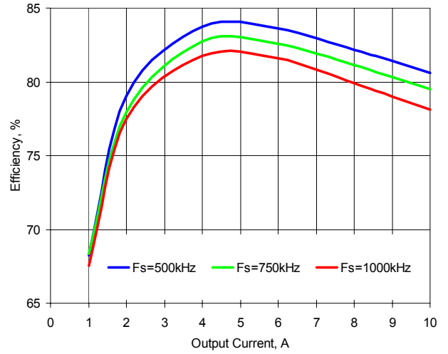
Figure 8. Efficiency vs. Load. V in =5V, V out =1.2V
