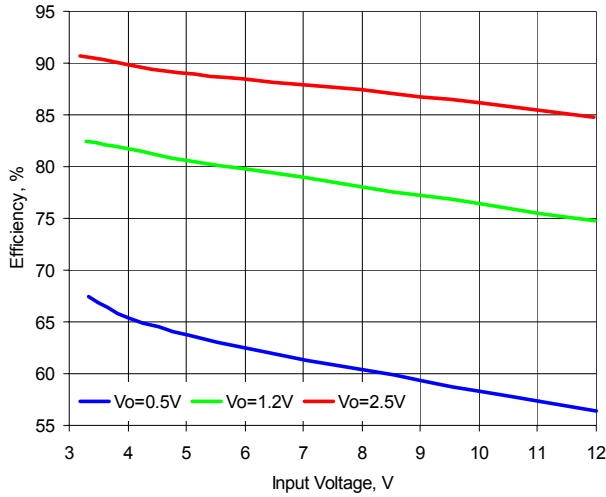
Figure 6. Efficiency vs. Input Voltage. I out =10A, F sw =500kHz
