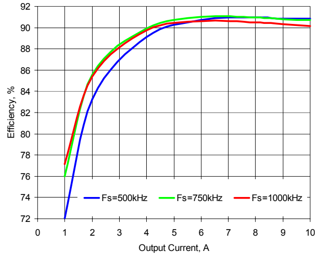
Figure 9. Efficiency vs. Load. V in =12V, V out =5V
