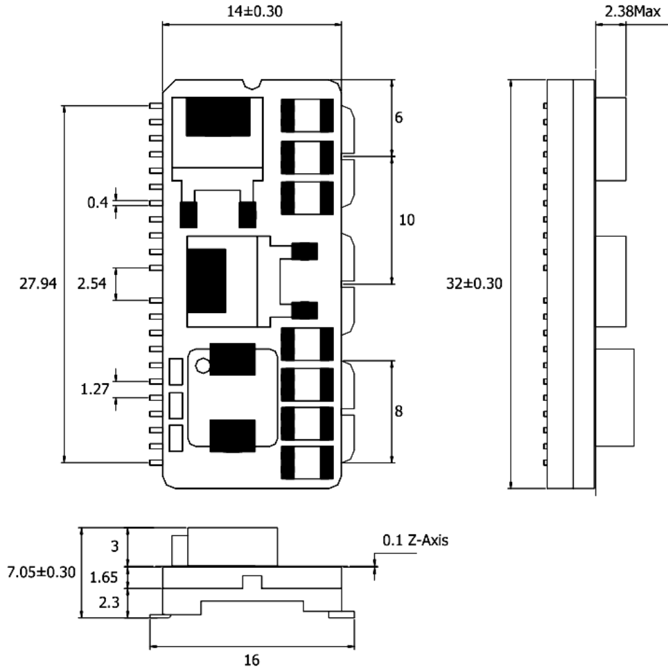
Figure 58. Mechanical Drawing
