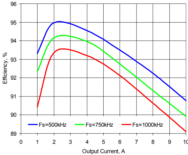
Figure 7. Efficiency vs. Load. V in =3.3V, V out =2.5V
