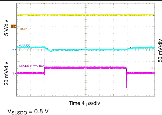
Figure 83. 0.8 V LSLDO Load Transient, 0 to 10 mA
