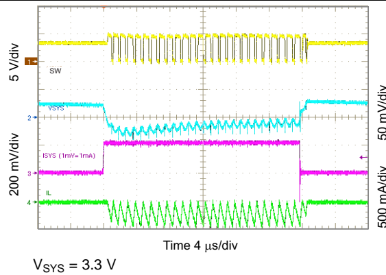
Figure 78. 3.3 V_{SYS} Load Transient, 0 to 200 mA
