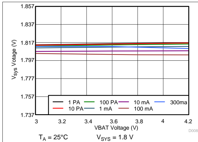
Figure 58. 1.8 V_{SYS} Line Regulation
