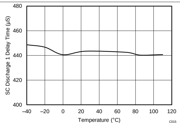
Figure 16. Short Circuit Discharge 1 Delay Time vs. Temperature
