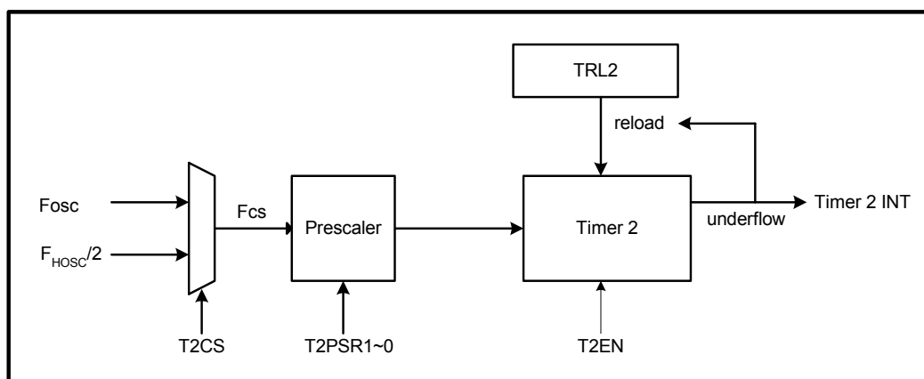
Figure 8-3 Timer 2 Function Block Diagram
