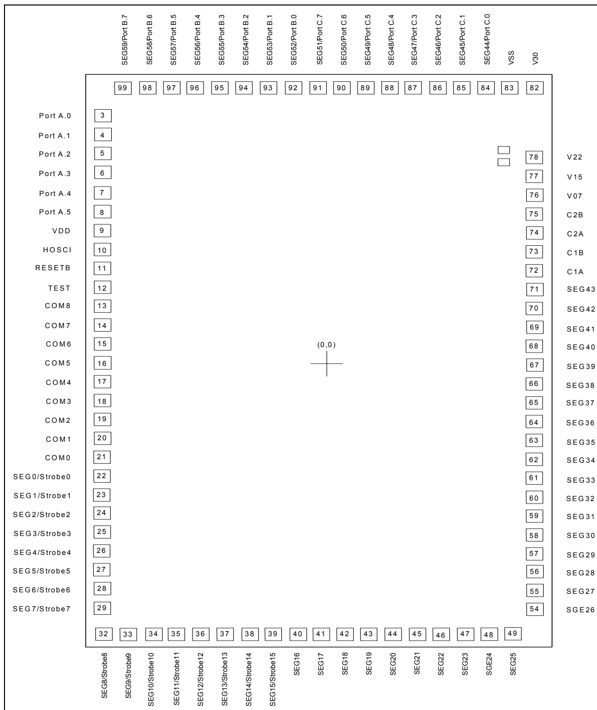
Figure 13-1 ePS6002 88 Pin-Out
