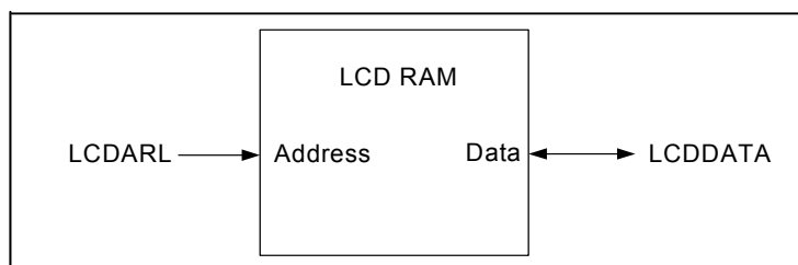
Figure 8-10 LCDDATA Register Access through LCD RAM
