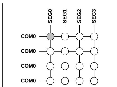
Figure 8-14a LCD COM & SEG Waveform Matrix
