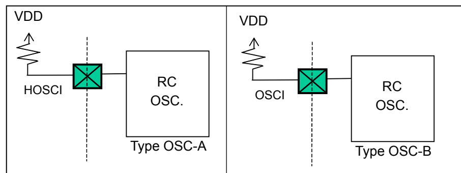
Figure 10-1c Oscillator Pin Type Circuit Diagram
