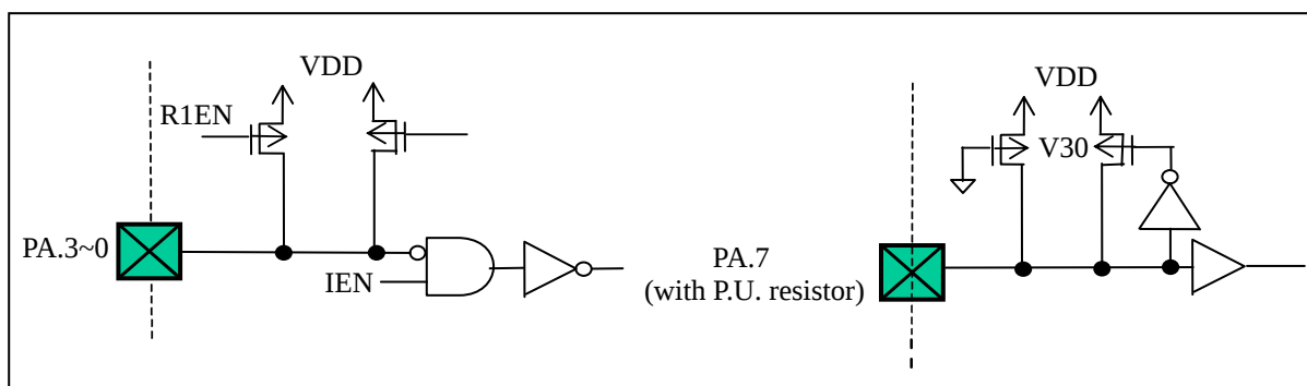
Figure 10-1d Input Pin Type Circuit Diagram
