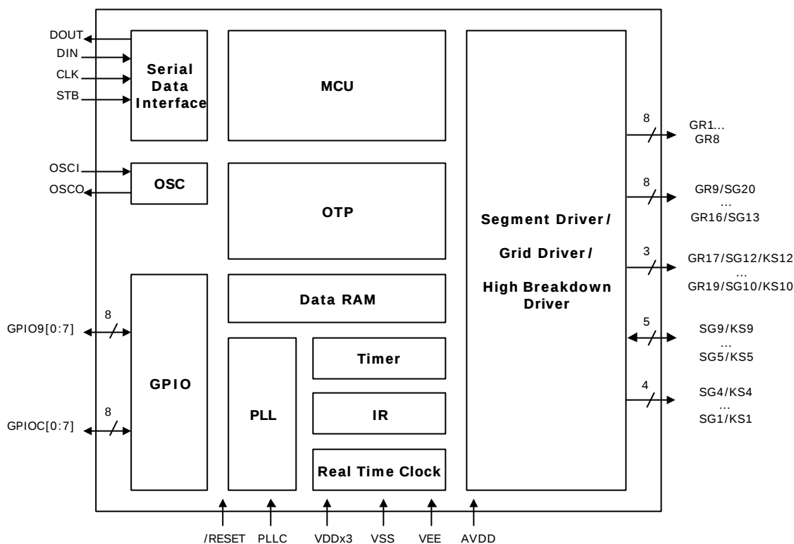
Fig.2a Block diagram
