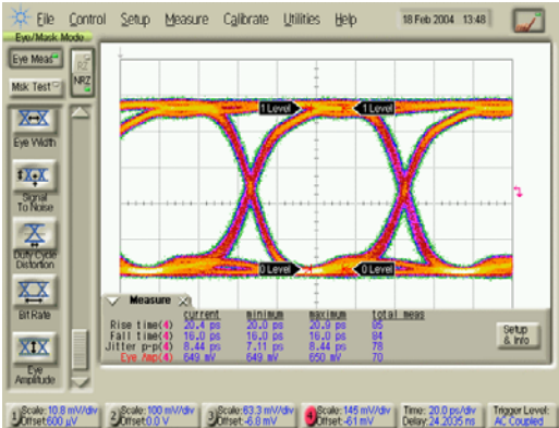
Bit rate: 12.5 Gb/s Vin = +/-200 mVpp, Vout = +/-644 mVpp
