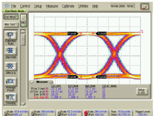
Bit rate: 12.5 Gb/s Vin=+/-8 mVpp, Vout=+/-1.1 mVpp
