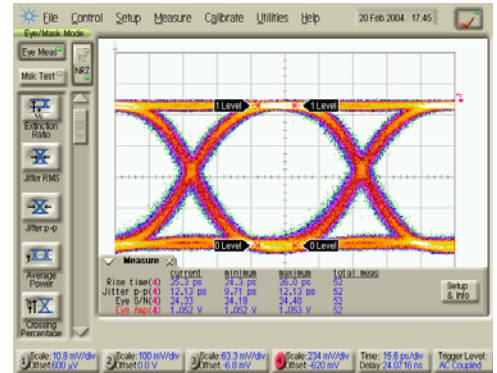
Bit rate: 12.5 Gb/s Vin=+/-5 mVpp, Vout=+/-1Vpp
