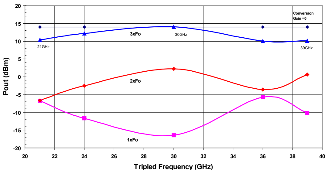
Figure 5. Measured Tripler Performance.
