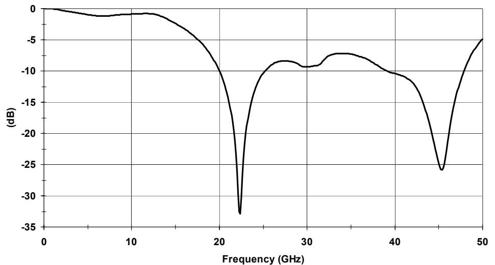
Typical Output Return Loss Vs. Frequency Bias V_D=3.5 V, I_{DQ}=350 mA
