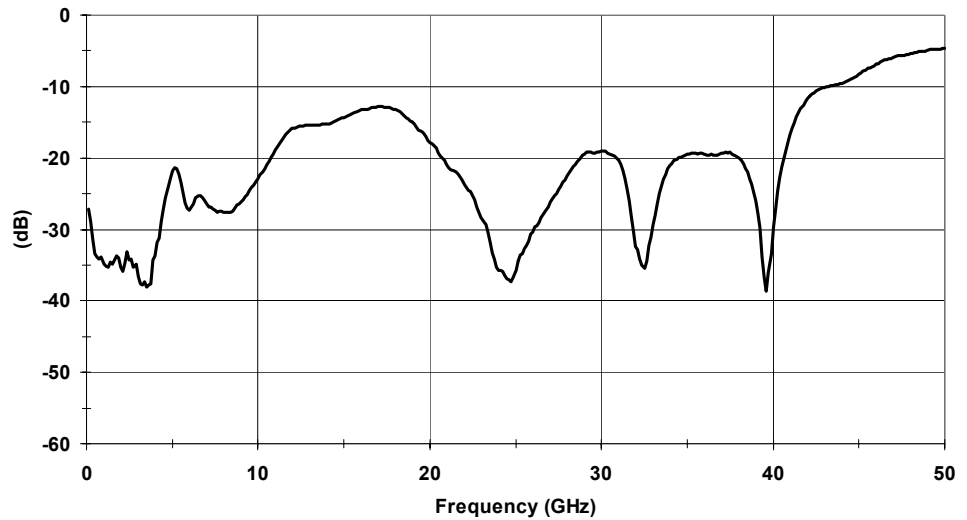
Typical Input Return Loss Vs. Frequency Bias V_D=3.5 V, I_{DQ}=350 mA
