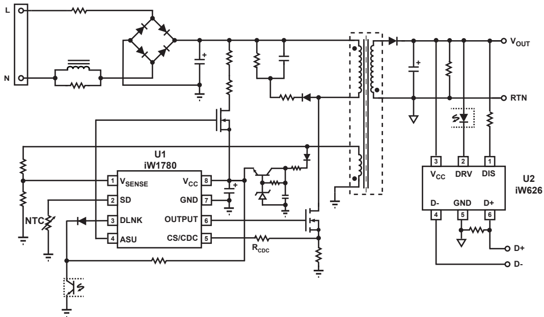
Figure 9.5: Typical Application Circuit with V_{CC} LDO and Opto-Coupler Acceleration
