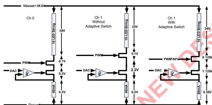
Figure 9.1 : Power Loss Improvement Through Adaptive Switch Method
