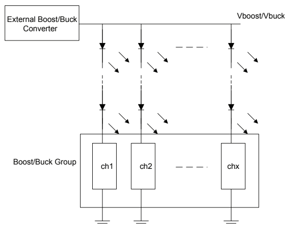
Figure 9.9 : iW7032 Boost/Buck Groups
