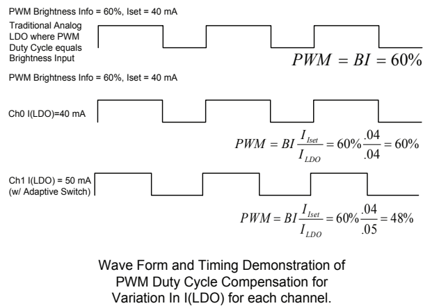
Figure 9.2 : PWM Duty Cycle Compensation
