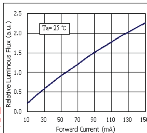
Figure 9.3 : Optical Luminance vs. Forward Current in an LED
