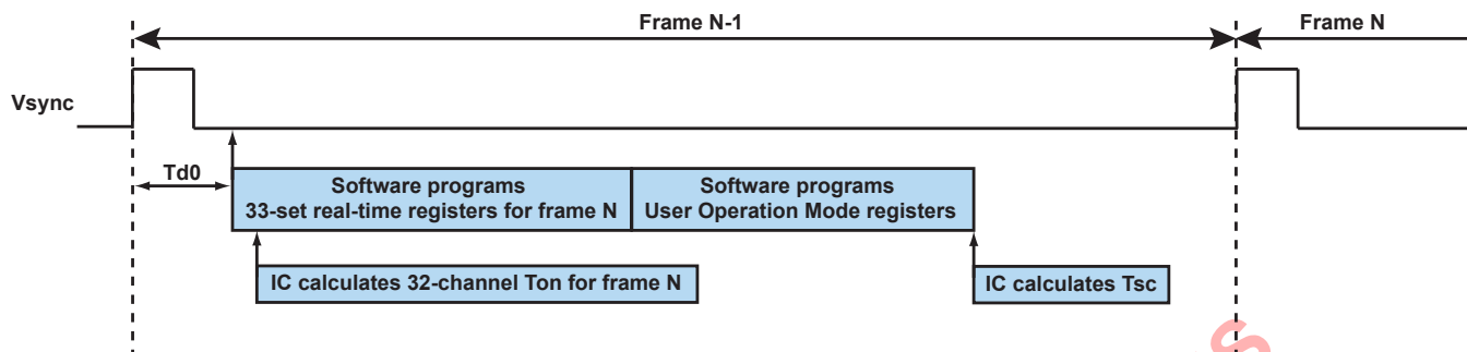
Figure 17.1 : User Operation Mode Register Update Timing
