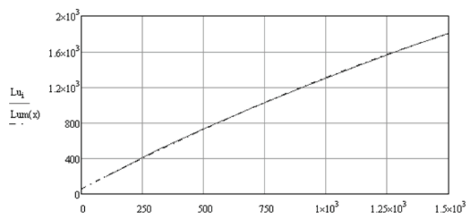
Figure 9.4 : Scaled Diode Curve
