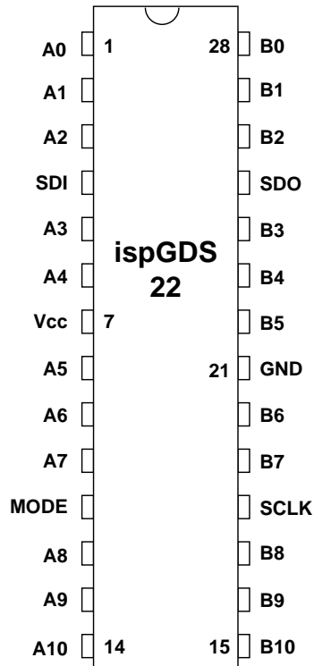
28-Pin DIP
