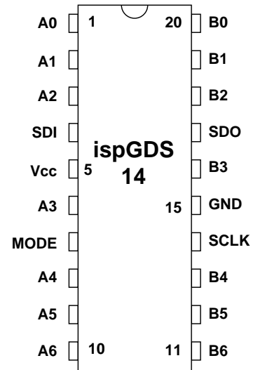
20-Pin DIP
