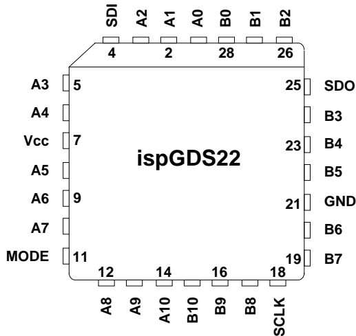
28-Pin PLCC
