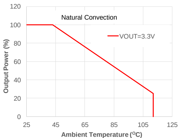
Power Derating V_{IN} = 12V , V_{OUT} = 3.3V
