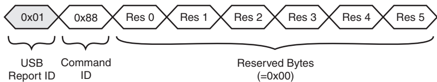
Figure 12-10.Command Packet Format
