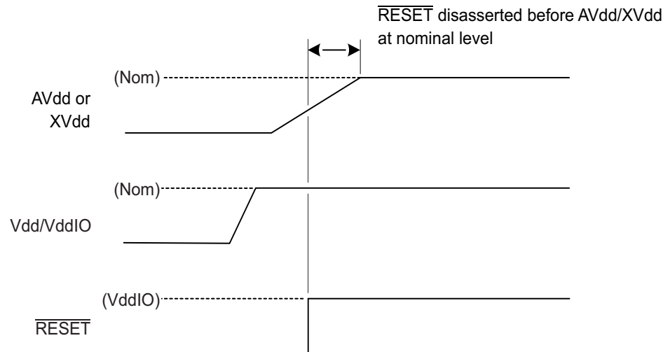
Figure 7-2. Power Sequencing on the mXT2954T2 – Late rise on AVDD or XVdd
