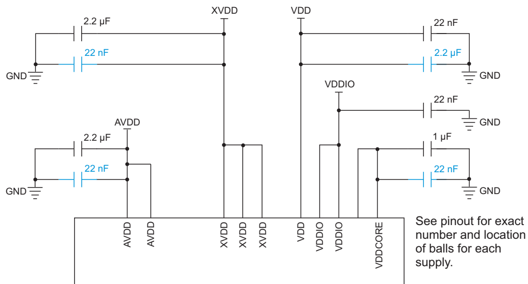
Figure 3-1. Additional Recommended Decoupling Capacitors
